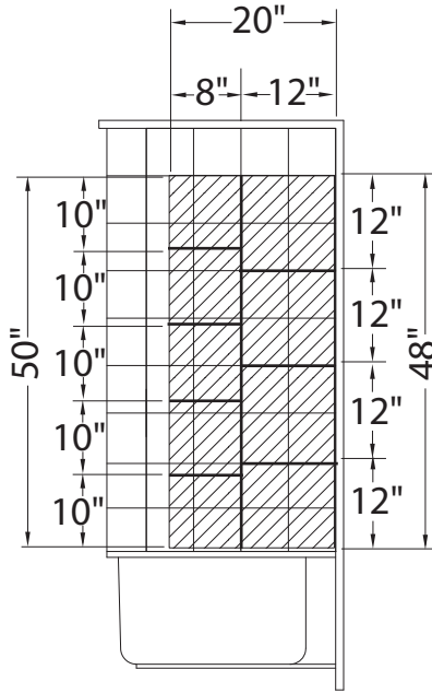
LEFT WALL Reinforcement
