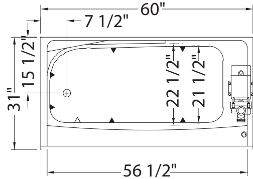
BACK WALL Reinforcement
