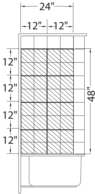
RIGHT WALL Reinforcement
